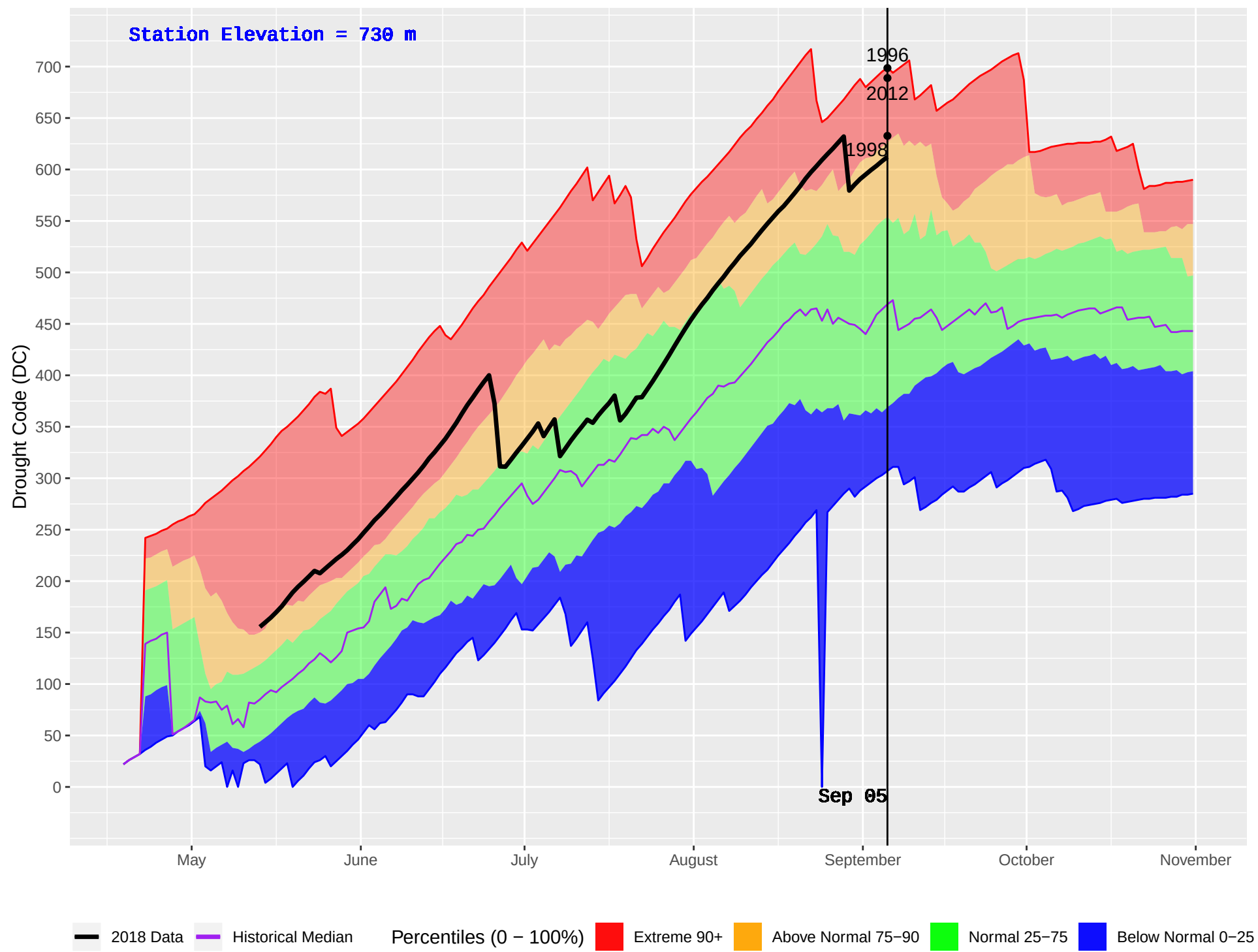
BOYA LAKE (445) : Historical (1985–2016) and Current (2018) Daily Drought Code (DC)
