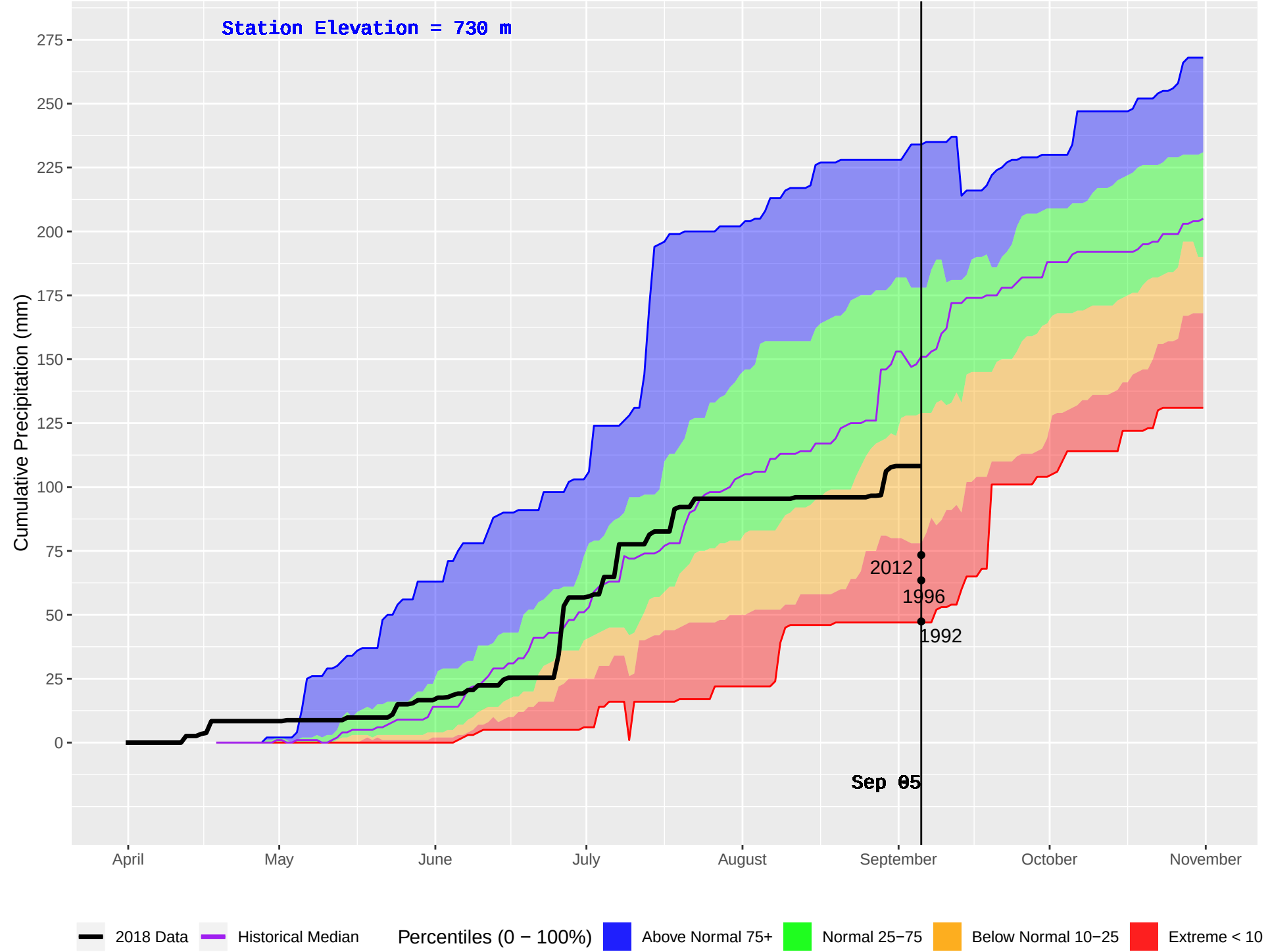
BOYA LAKE (445) : Historical (1985–2016) and Current (2018) Daily Cumulative Precipitation
