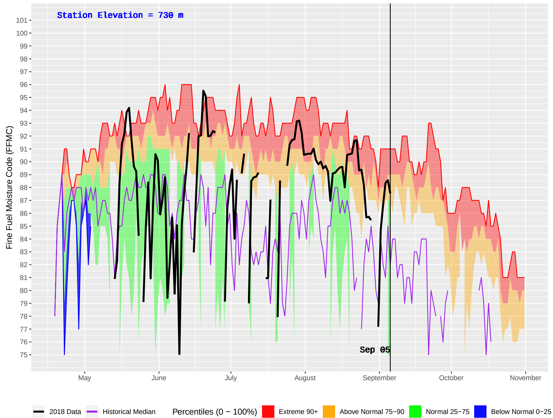
BOYA LAKE (445) : Historical (1985–2016) and Current (2018) Daily Fine Fuel Moisture Code (FFMC)
