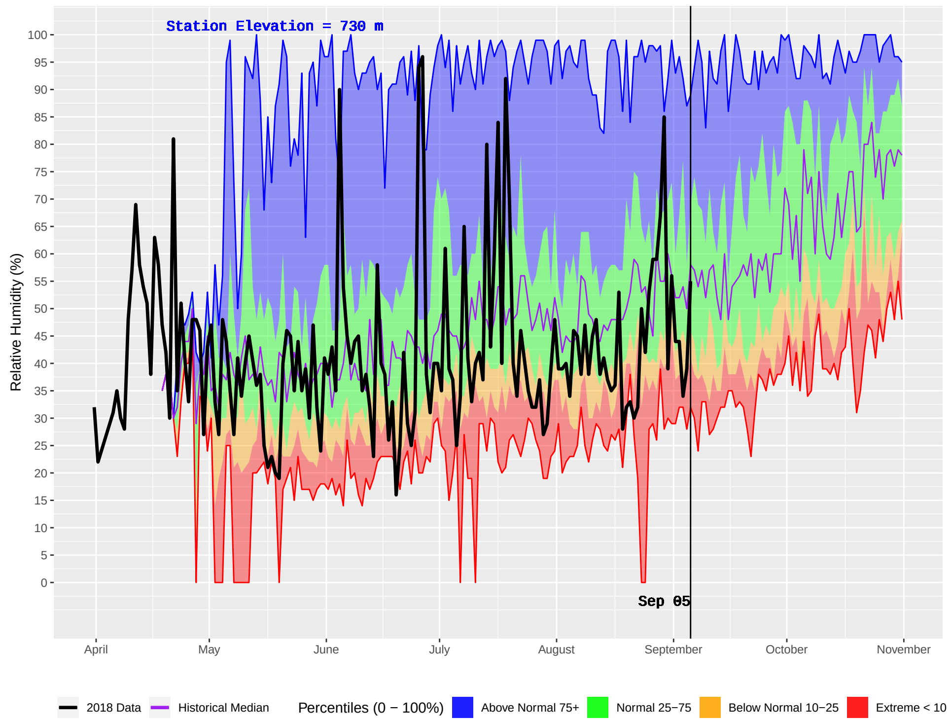
BOYA LAKE (445) : Historical (1985–2016) and Current (2018) Daily Relative Humidity
