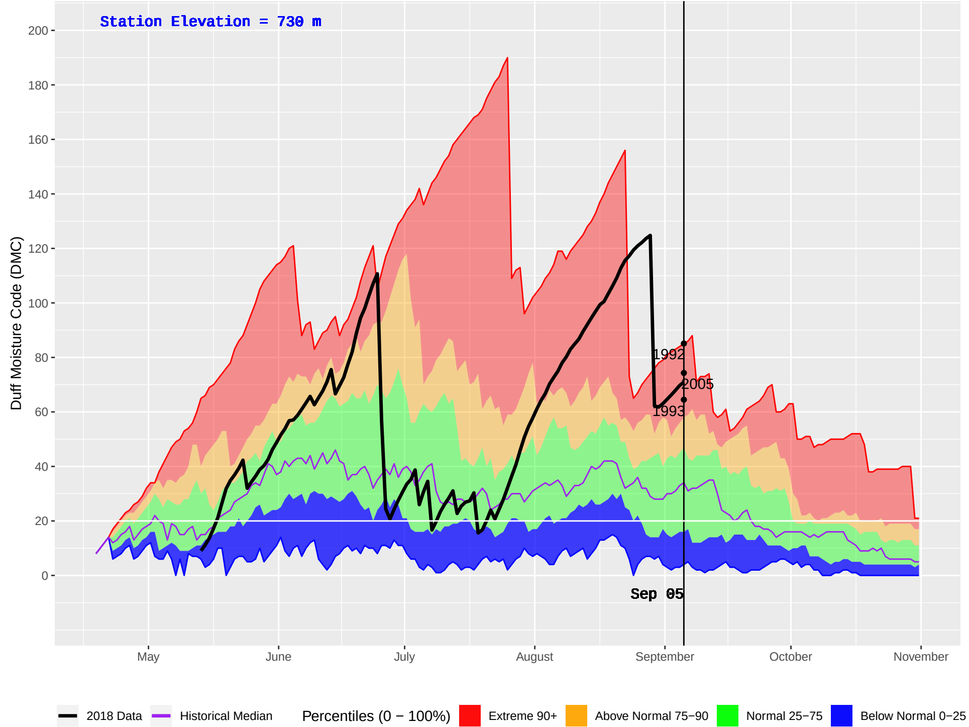
BOYA LAKE (445) : Historical (1985–2016) and Current (2018) Daily Duff Moisture Code (DMC)
