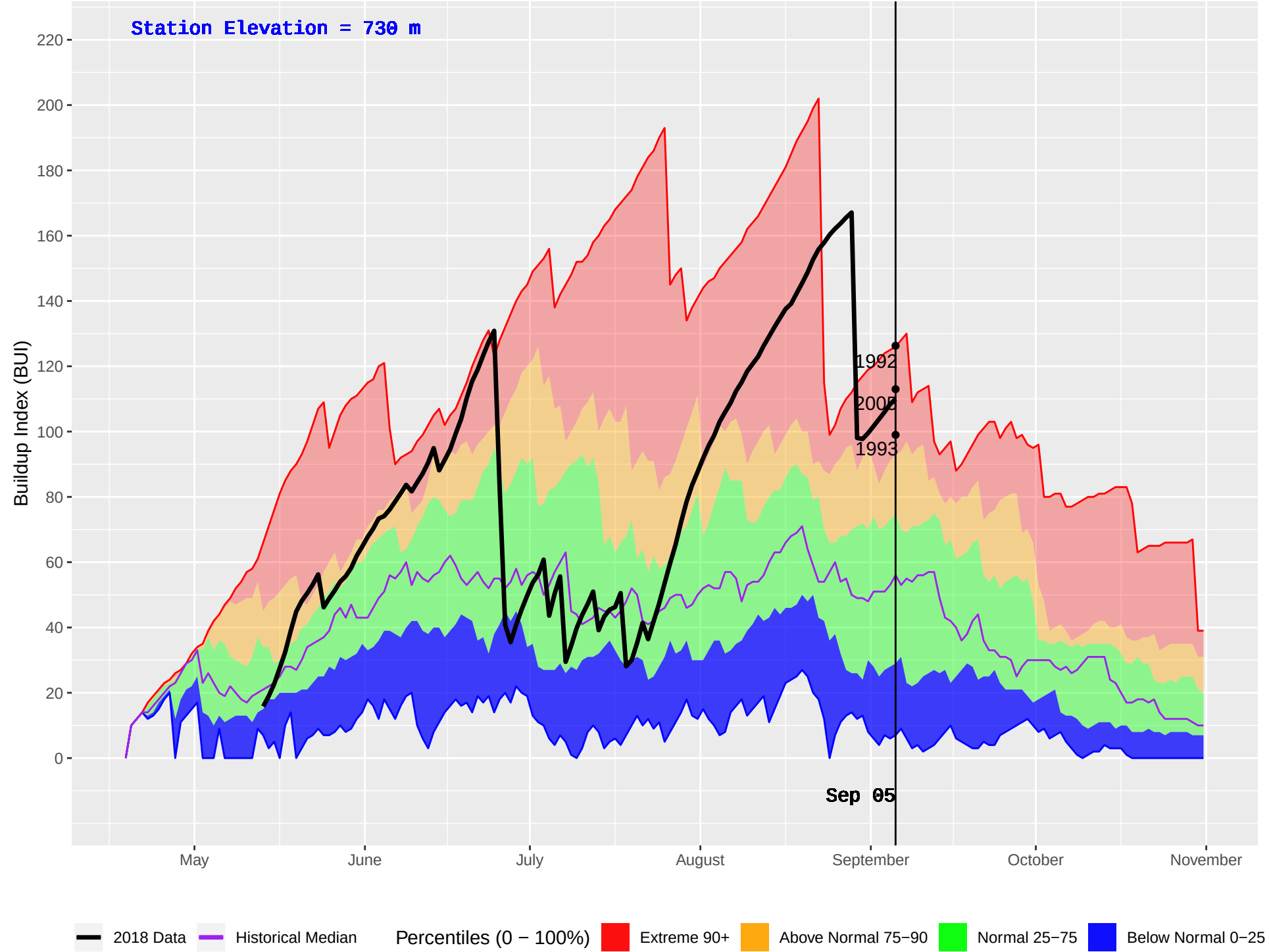
BOYA LAKE (445) : Historical (1985–2016) and Current (2018) Daily Buildup Index (BUI)
